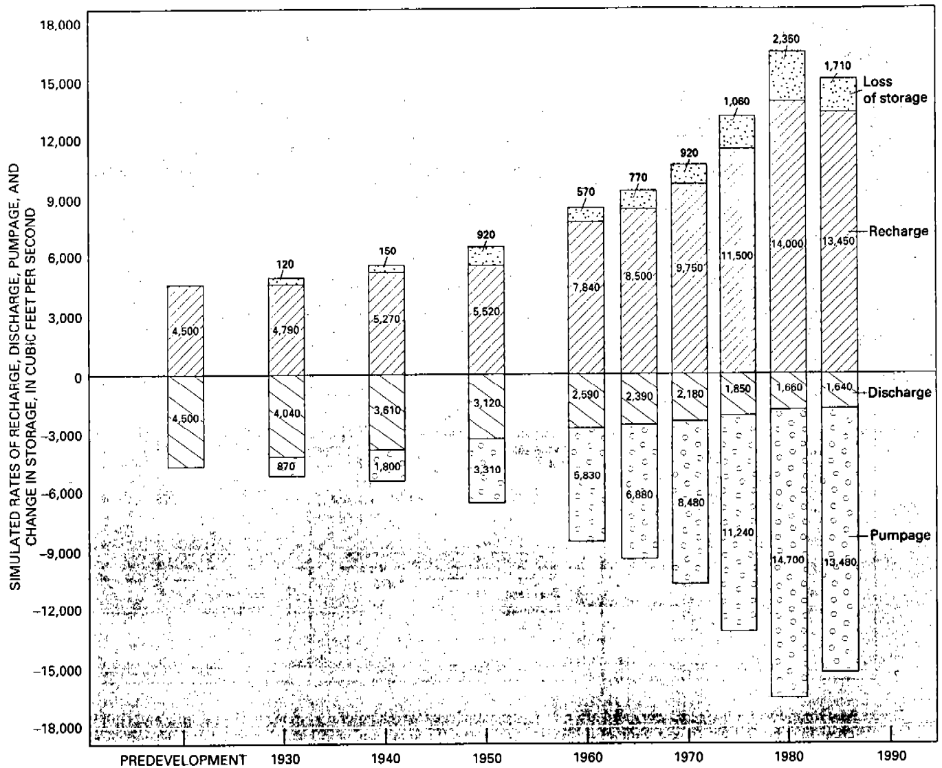
FIGURE 7.—Change in simulated regional ground-water budget of the Gulf Coastal Plain aquifer systems from predevelopment to 1985 (modified from Williamson, in press, fig. 45).
