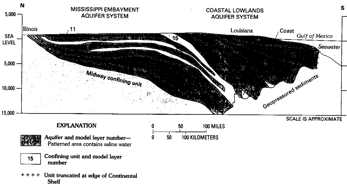
FIGURE 4.—Aquifers and confining units and designation of layers in the regional flow model of the Gulf Coastal Plain aquifer systems (from Williamson, in press, fig. 10A).
