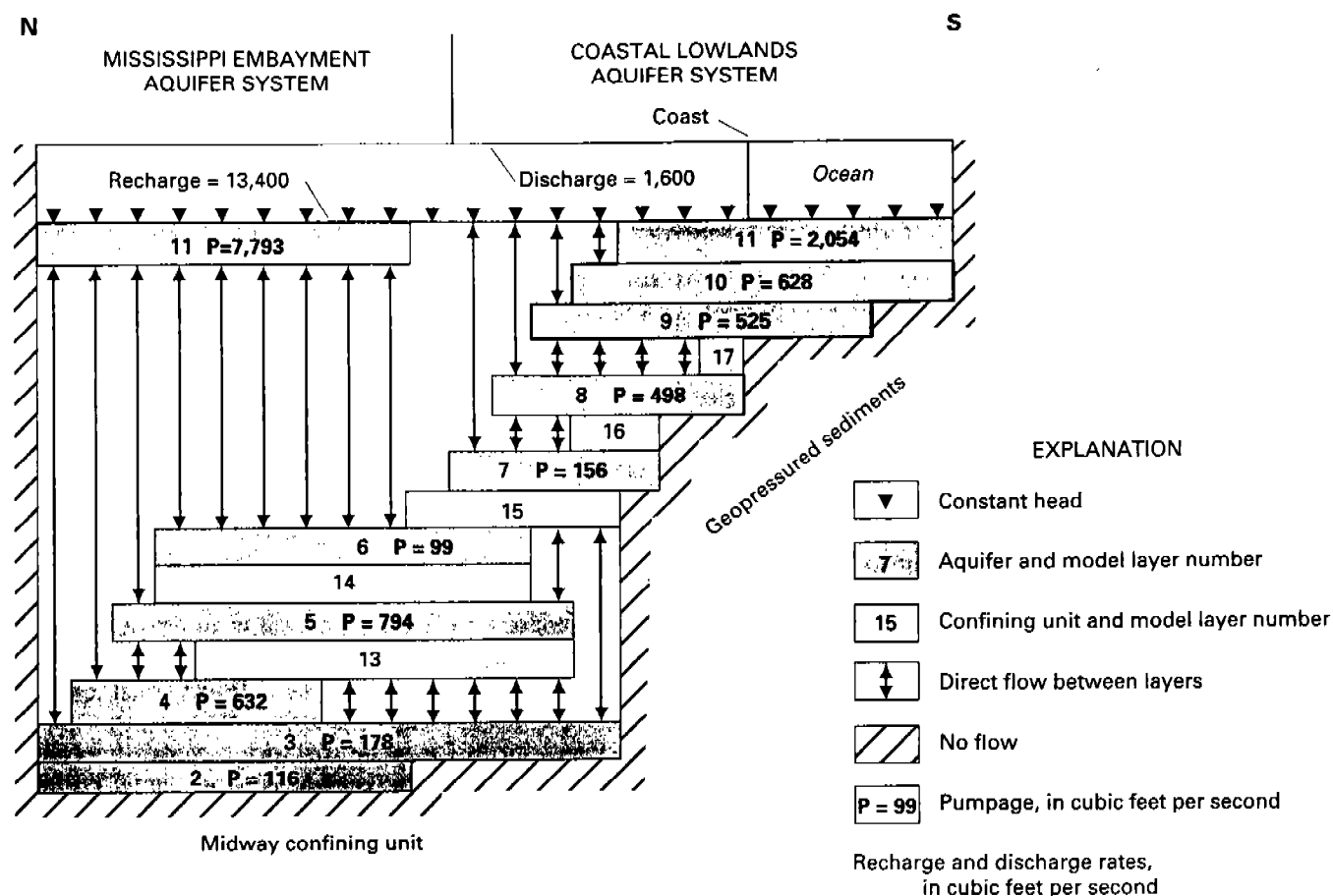
FIGURE 5.—Vertical structure of the regional flow model of the Gulf Coastal Plain aquifer systems and simulated 1985 rates of recharge, discharge, and pumpage (modified from Williamson, in press, fig. 10B).
