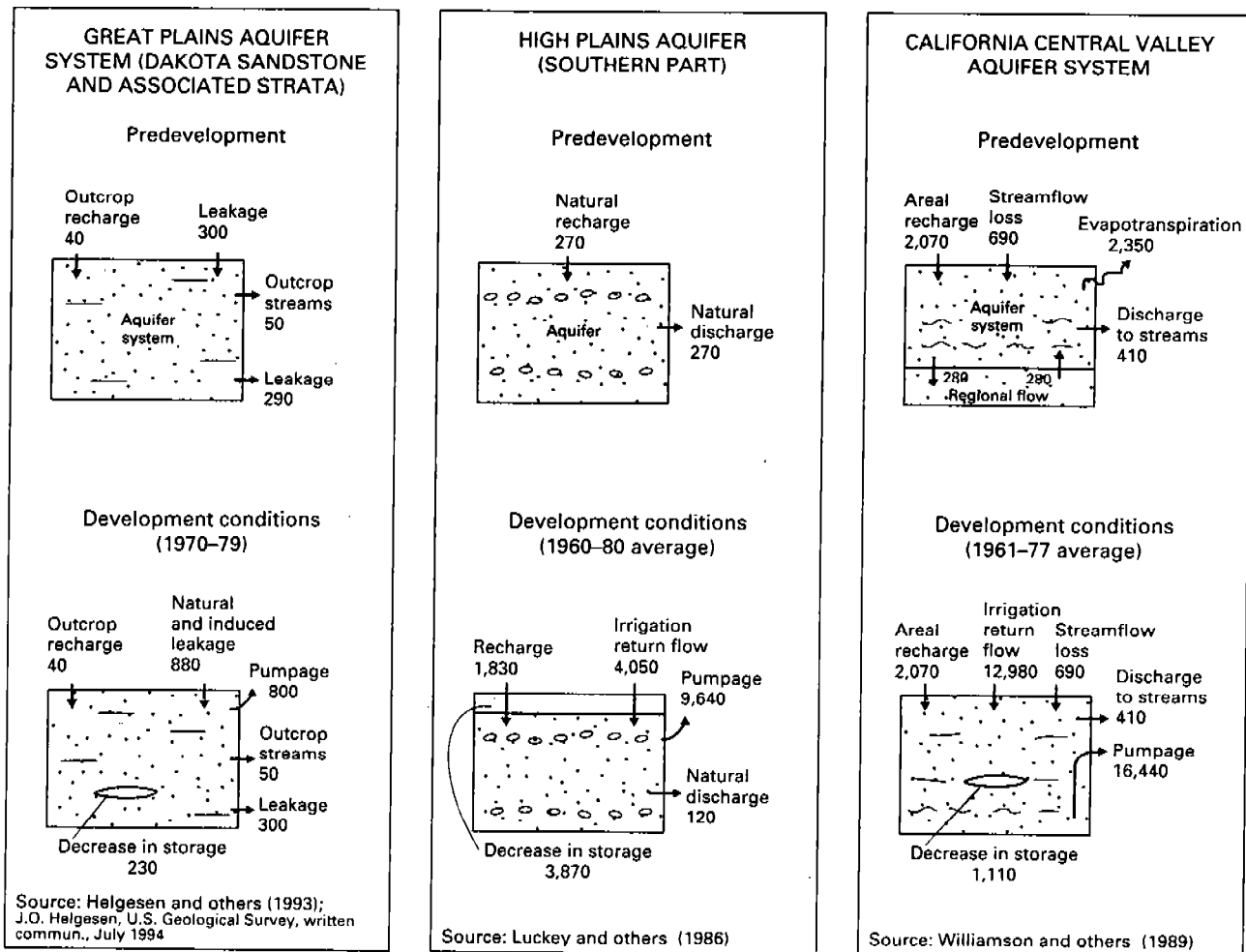
FIGURE 10.—Ground-water budgets before and after development of clastic-rock aquifer systems in the Central and the Western United States. Values in cubic feet per second. Sum of outflows may not exactly equal sum of inflows as a result of independent rounding.
