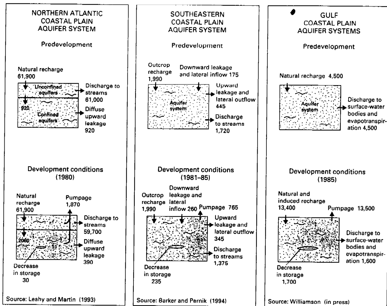
FIGURE 6.—Ground-water budgets before and after development of clastic-rock aquifer systems in the Atlantic and Gulf Coastal Plains. Values in cubic feet per second. Sum of outflows may not exactly equal sum of inflows as a result of independent rounding.
