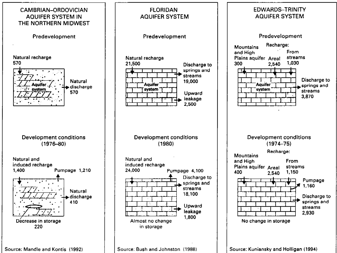
FIGURE 8.—Ground-water budgets before and after development of carbonate-rock aquifer systems in the Midwestern and Southern United States. Values in cubic feet per second. Sum of outflows may not exactly equal sum of inflows as a result of independent rounding.
