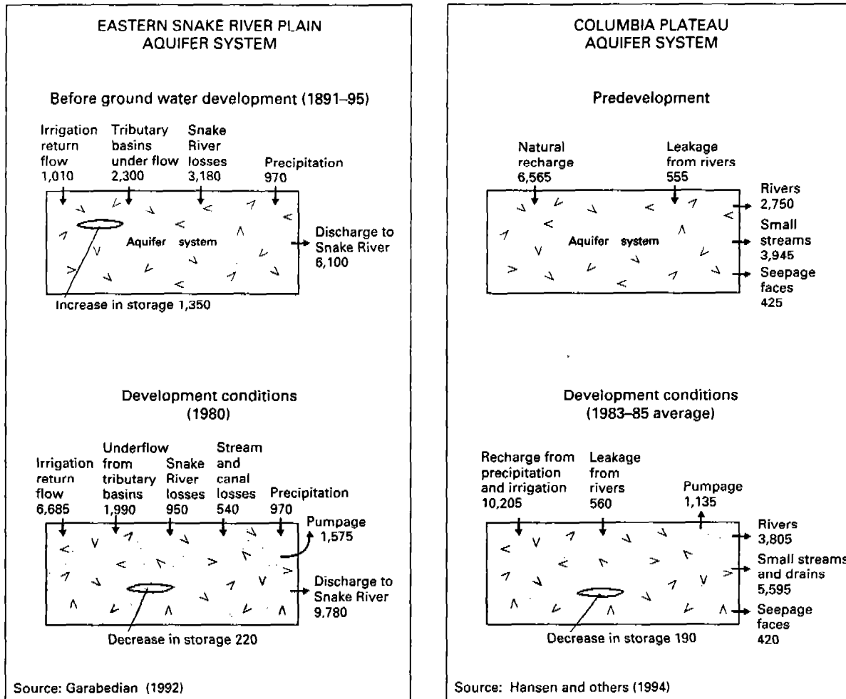
FIGURE 11.—Ground-water budgets before and after development of basaltic-rock aquifer systems in the Pacific Northwest. Values in cubic feet per second. Sum of outflows may not exactly equal sum of inflows as a result of independent rounding.
